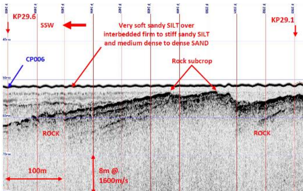
Figure 15: Interpreted SBP Seabed Profile
