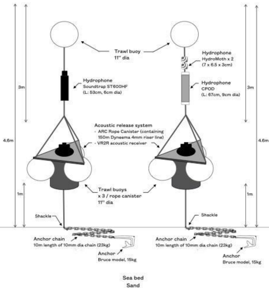
Mooring set up A
